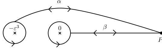
FIGURE 5.1. Generators of \pi_1(p^{-1}(\varepsilon), P)
