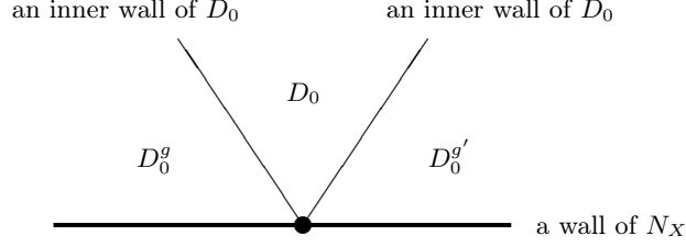
FIGURE 5.1. A D_0 -inner face that is not N_X -inner.
